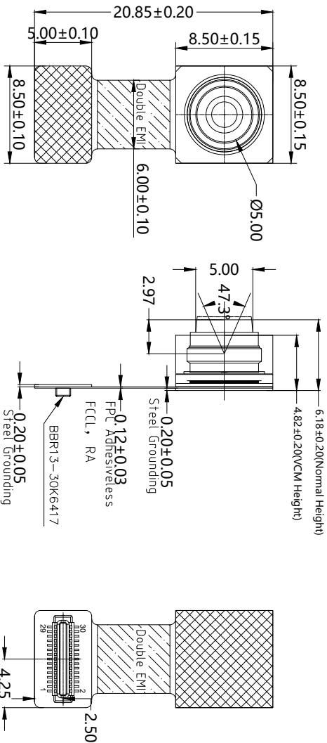
TOP VIEW
